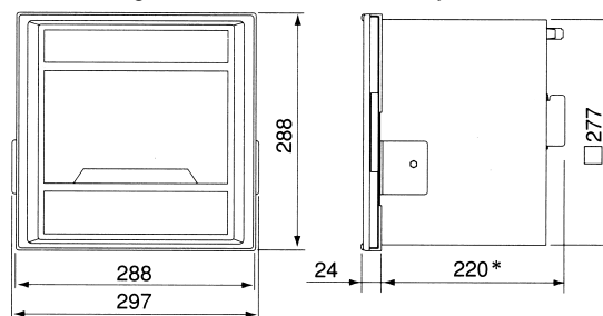
Panel cutout and minimum clearance for installation
