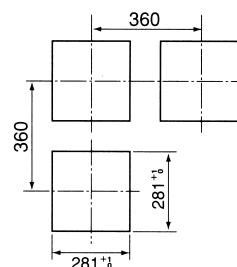
Panel cutout and minimum clearance for installation
